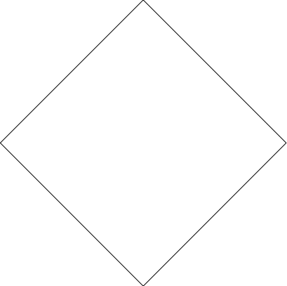
Amethyst
