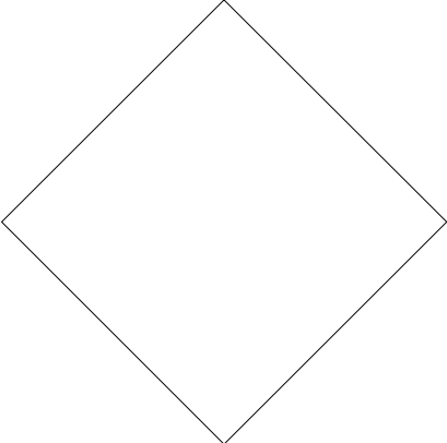
Rhodochrosite
