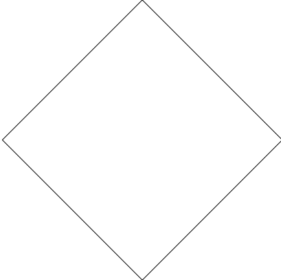
Tourmaline
